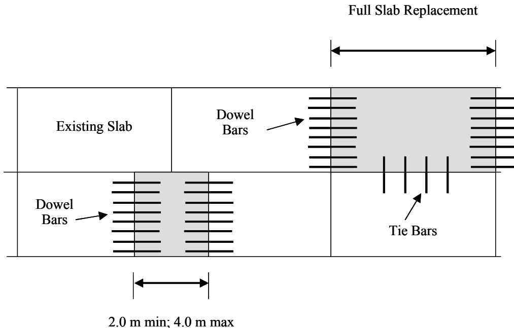
FIGURE 13. Example layout for full-depth repairs for a 2-lane section.
