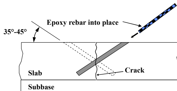
FIGURE 3. Stitched longitudinal crack.
