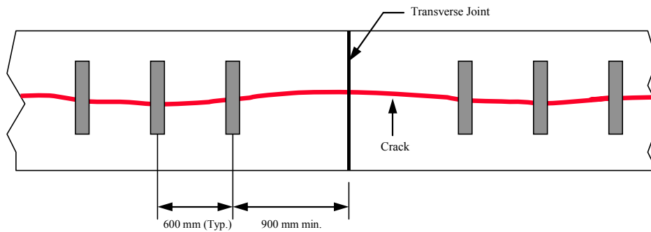
FIGURE 5 Typical spacing of dowels across a transverse crack.
