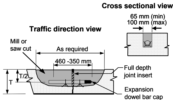
FIGURE 6 Dowel bar placement for load transfer retrofit.
